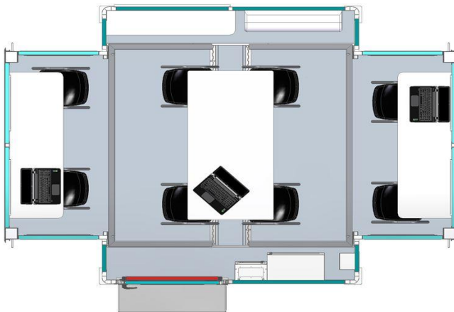
Top view of the “extended” module
