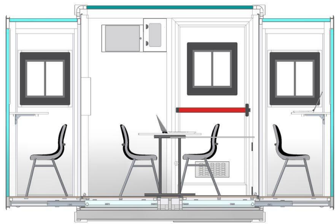
Vertical section of the “extended” module
