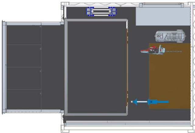
Top view in open "operating position"
