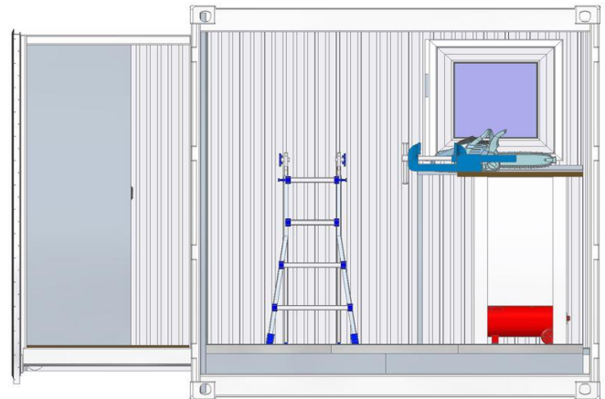
Vertical section with extended side body
